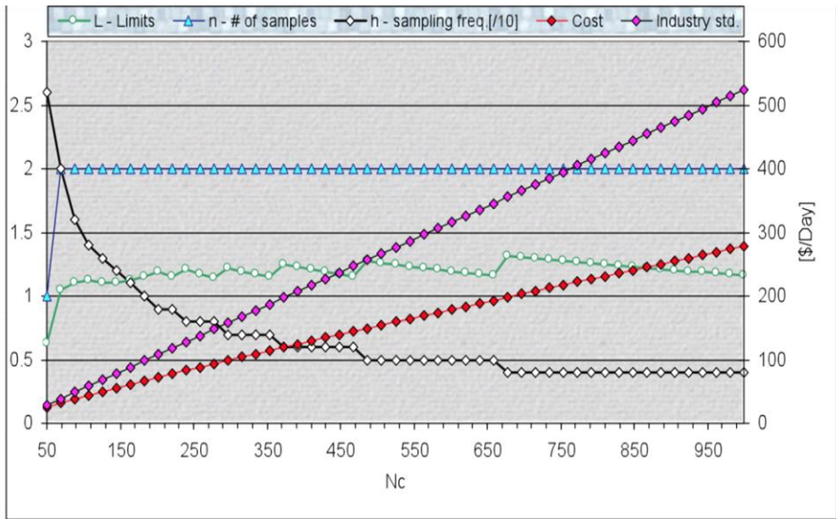
Figure 4. Effect of number of cows in the herd ( N_c ) on optimal sampling design and total quality costs per day; L = the optimal control limits for an X-bar chart, n = the number of samples to be taken at each sampling time, and h = the sampling frequency expressed in days/10. The cost is the total quality cost per day. The industry standard curve is the total quality cost for the herd if a conventional sampling design is used (i.e., n = 1 , h = 30 d, and L = 2 ). Note that for a herd of 1000 cows (becoming increasingly more frequent in the USA) the economic savings to using an optimal sampling design (bottom diamond line) vs. the conventional design (upper diamond line) exceeds 250 US$/d.
